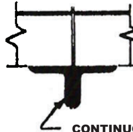
CONTINUOUS LINE LOUVER (Expansion Joint Approx. 10 O.C.)
